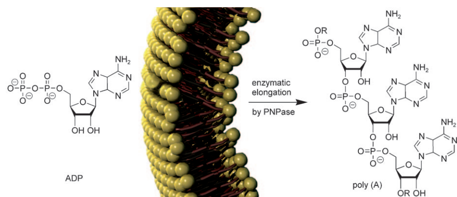
Scheme 1. ADP permeates across the vesicular bilayer into the interior space of oleic acid/oleate vesicles. Intra-protocellular enzymatic ADP elongation, catalyzed by polynucleotide phosphorylase (PNPase), results in poly(A), which stays in the extracellular medium. [45]
