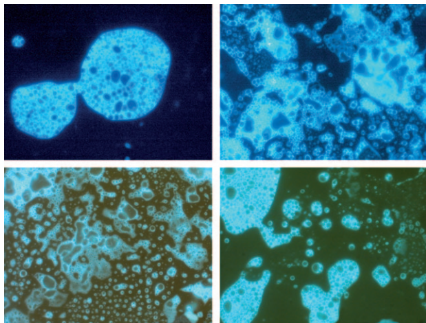
Figure 1. Residue droplets of a simulated precometary ice at pH 8.5 viewed by fluorescence microscopy and with 100-fold enlargement. The precometary ice was simulated by 0.8 MeV proton bombardment of amorphous ices of \text{H}_2\text{O} , \text{CH}_3\text{OH} , \text{NH}_3 , and \text{CO} (100:50:1:1) at 15 K in a high-vacuum chamber. [17] The gas composition was chosen as a simple mixture that reflects the composition and concentrations of the major components of interstellar ice. The four images were recorded with different filters and show different areas of the extract.
