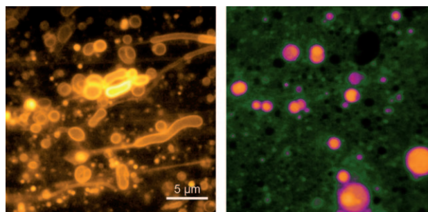
Figure 4. Left: Decanoic acid/decanol vesicles stained with fluorescent rhodamine; right: 600 mers of DNA encapsulated in vesicles of decanoic acid alone by the dehydration/rehydration method. The DNA was stained with 3,6-dimethylaminoacridine (acridine orange), a nucleic acid selective stain used to enhance the contrast in the microscopic image. Reprinted with permission from David Deamer, UC Santa Cruz.
