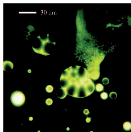
Figure 2. Compounds from meteorites seen in a new light: pyranine dye encapsulated in vesicles made from an extract of the Murchison meteorite. Vesicles show interior spaces with sizes in the micrometer range; oil droplets and inverse emulsions are also visible. [15] Copyright (2001) National Academy of Sciences, USA.
