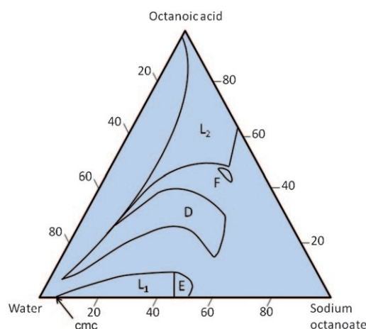
Figure 3. Ternary phase diagram for the sodium octanoate, octanoic acid, and water system at 20 °C expressed in wt%. The isotropic solution region L_1 represents an aqueous solution, and the isotropic solution region L_2 represents the solution of sodium octanoate and water in octanoic acid. E and F (liquid-crystalline two-dimensional hexagonal phase regions) are normal and inverse, respectively. The lamellar liquid-crystalline region D occurs in the center of the diagram. The phase diagram of the ternary system was shown to be very similar for longer chain length fatty acids as well as for the potassium carboxylate, carboxylic acid, and water system. [44]
